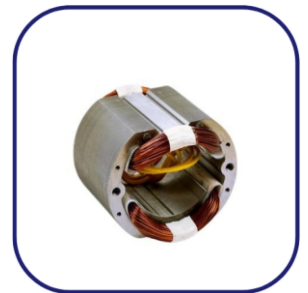
7614-NB-Field Coil
